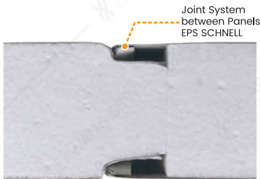
Tebal 100mm HRM SN03 S
