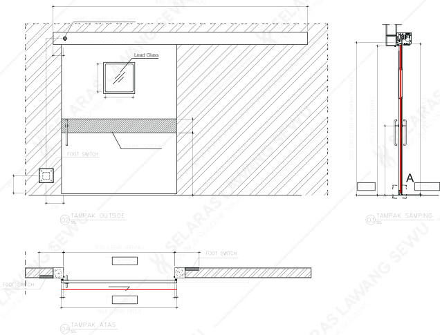
HERMETIC SINGLE
